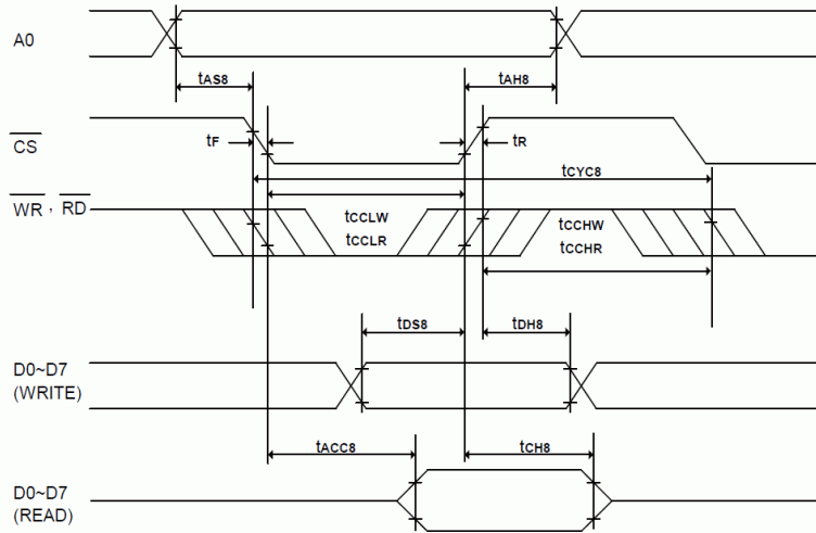
(1) System buses Read/Write characteristics 1 (For the 8080 Series Interface MPU)
