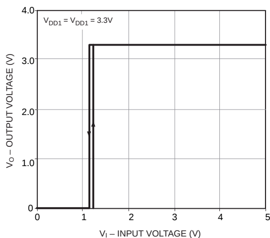
Figure 2. Typical Output Voltage vs. Input Voltage (Channel A & B)
