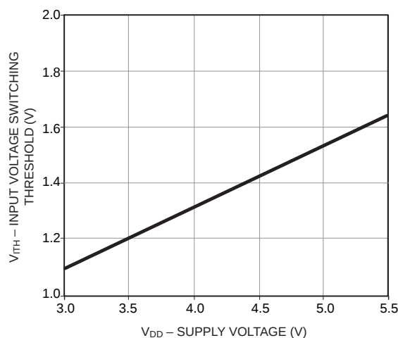
Figure 3. Typical Input Voltage Switching Threshold vs. Input Supply Voltage (Channel A & B)
