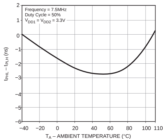
Figure 5. Typical t_{PHL} - t_{PLH} vs. Ambient Temperature (Channel A & B)
