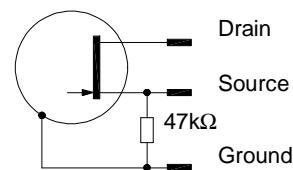
Fig.1: Test circuit
