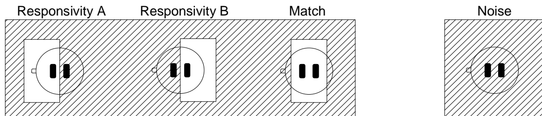
Fig.4.: Responsivity measurement
