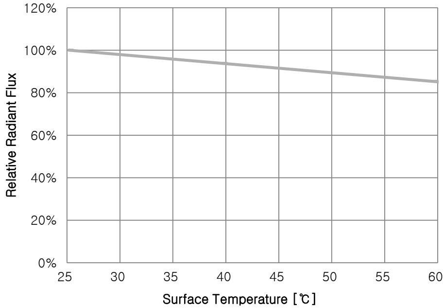
Fig 5. Surface Temperature vs. Relative Radiant Flux, I_F=30\text{mA}
