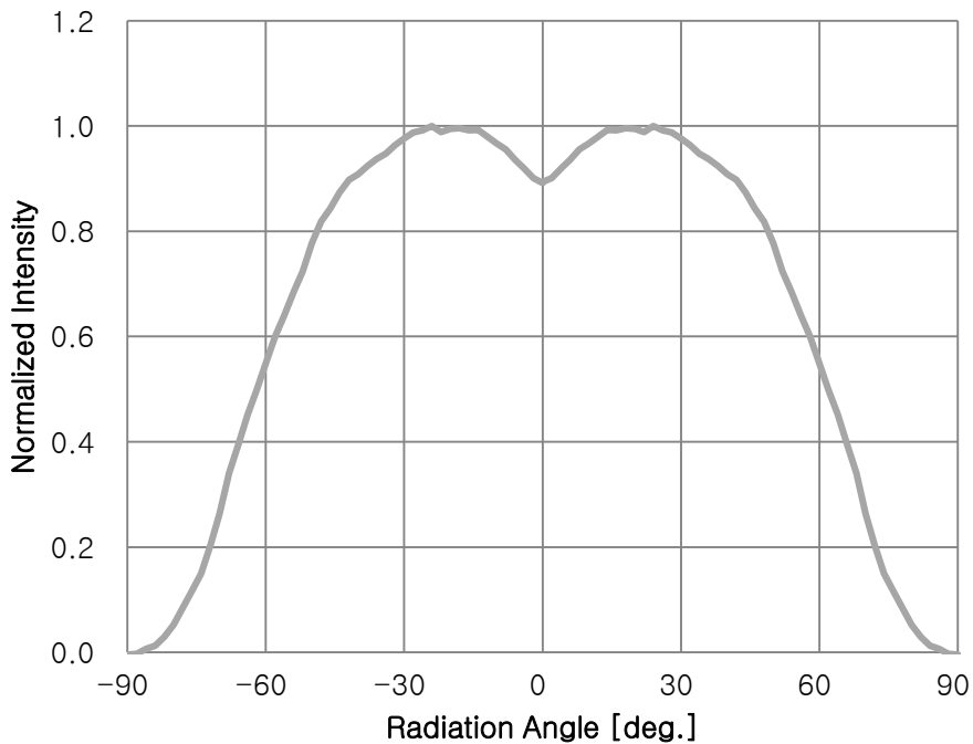
Fig 8. Typical Spatial Distribution, I_F=30\text{mA}
