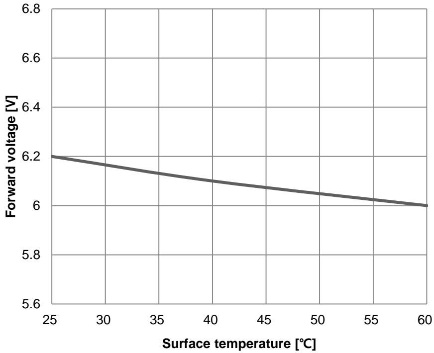
Fig 7. Surface Temperature vs. Forward Voltage, I_F=30\text{mA}
