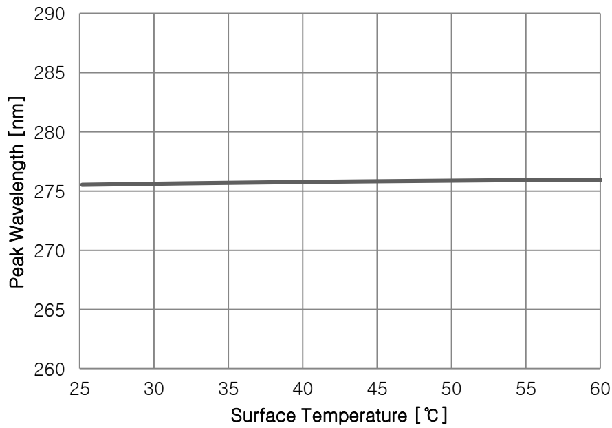
Fig 6. Surface Temperature vs. Peak Wavelength, I_F=30\text{mA}
