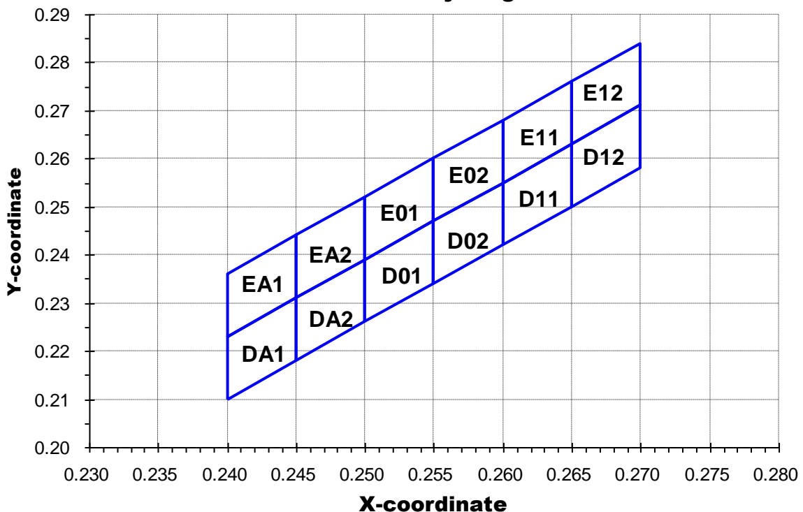
C. I. E. 1931 Chromaticity Diagram @20mA
