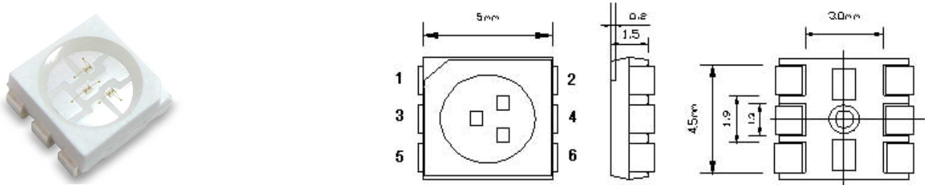
5050 TOP VIEW SMD
