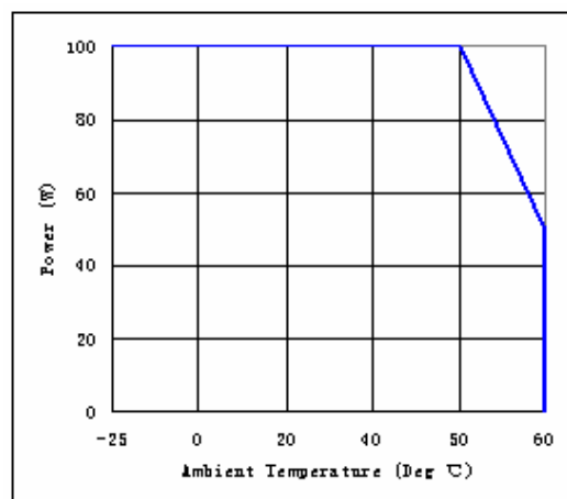
Derating Curve
