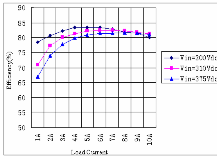
Typical Efficiency
