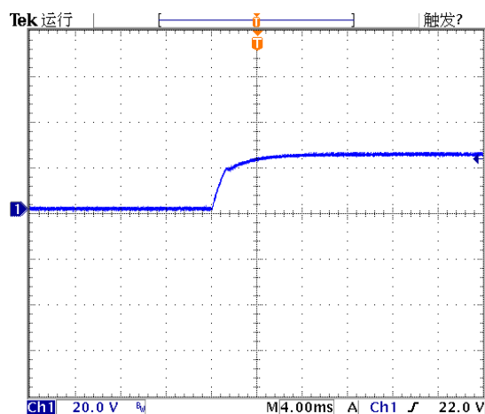
Typical Start-up
