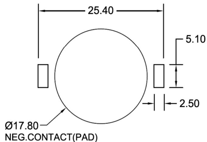
(MOUNTING PAD LAYOUT)
