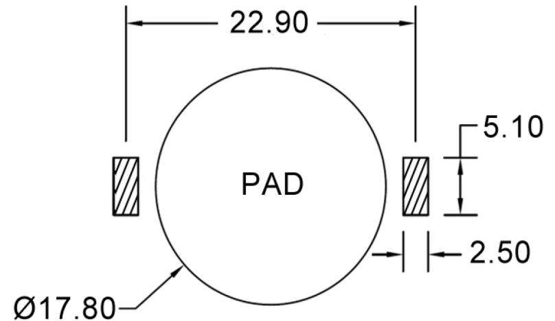
MOUNTING PAD LAYOUT
