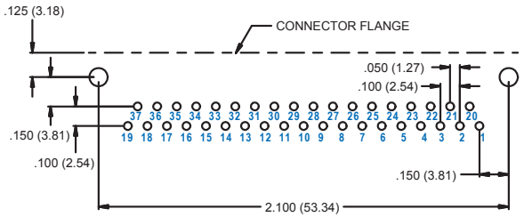
37 PIN M83513/16-F
