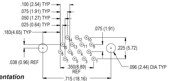
15 PIN M83513/28-B
