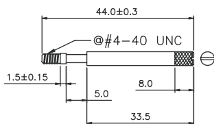
Long screw
