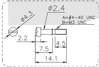
Short screw
