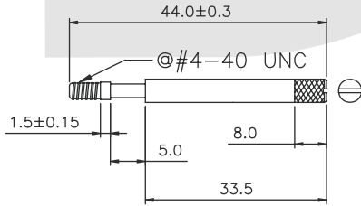
Long screw
