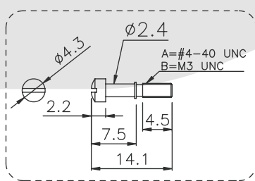
Short screw
