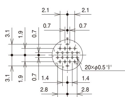
Size 9, 20 conductors
