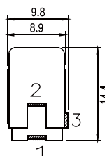
TERMINAL NUMBERS
