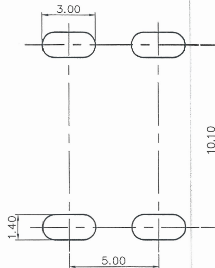
PCB LAYOUT
