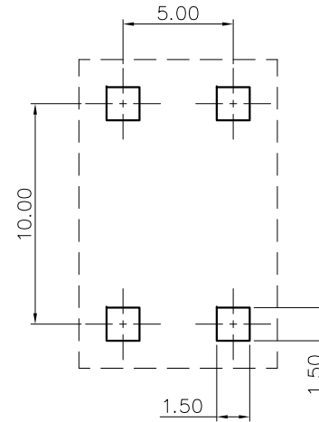
PCB LAYOUT
