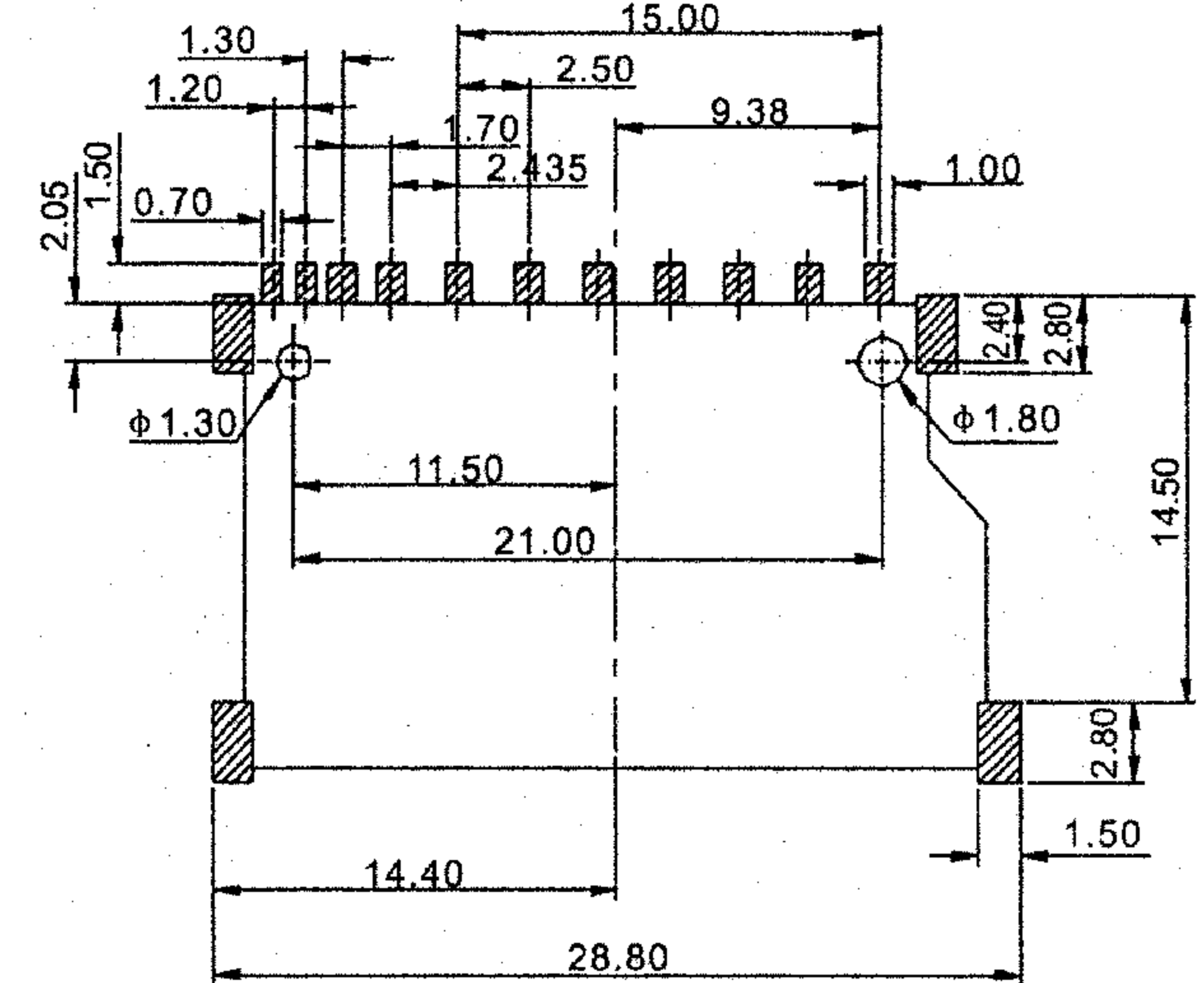
SUGGESTED PCB LAYOUT GENERAL TOLERANCE: \pm 0.05
