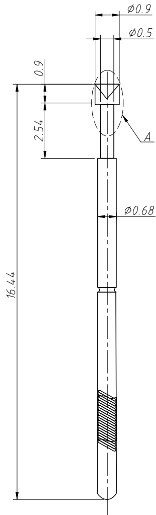
Needle Bar
