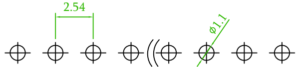
Recommended PCB Layout (PCB TOLERANCE ±0.1)
