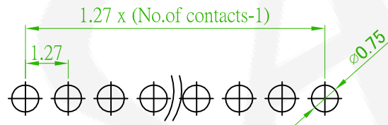
Recommended PCB Layout (PCB TOLERANCE ±0.1)
