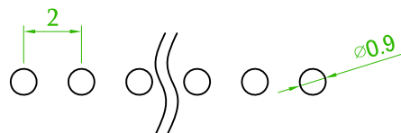
Recommended PCB Layout (PCB TOLERANCE ±0.1)
