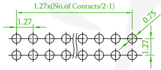
Recommended PCB Layout (PCB TOLERANCE ±0.1)
