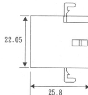
5H5030M1-104WBL00D01 1*4Pin With Ear
