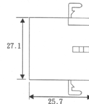
5H5030M1-105WBL00D01 1*5Pin With Ear
