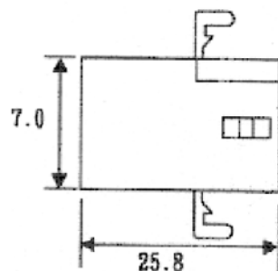
5H5030M1-103WBL00D01 1*3Pin With Ear
