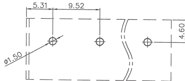
PCB LAYOUT
