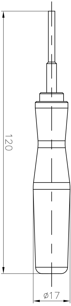
Contact removal tool Application: 10A Crimp contacts
