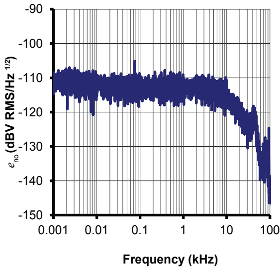
Figure 10: Typical output RMS noise voltage spectral density e_{no} with R_M = 50 \Omega
