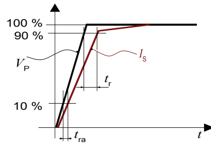
Figure 13: Response time t_r and reaction time t_{ra}
