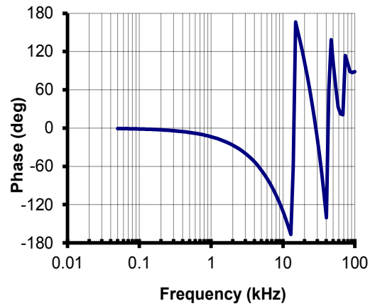
Figure 9: Typical frequency and phase response
