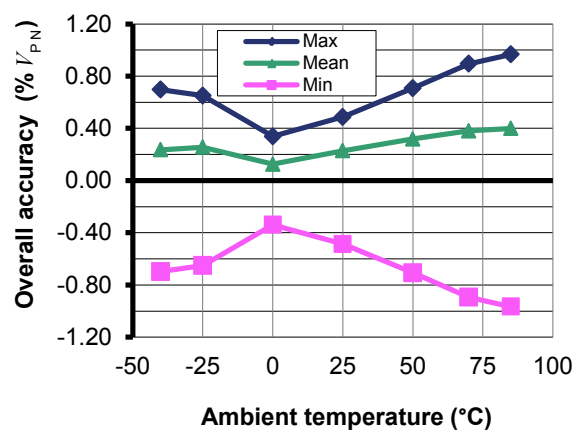
Figure 4: Overall accuracy in temperature
