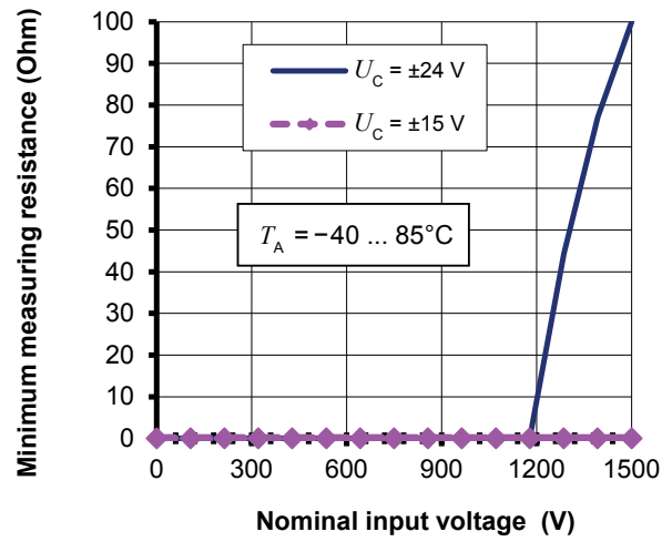
Figure 2: Minimum measuring resistance For T_A under 80\text{ }^\circ\text{C} , the minimum measuring resistance is 0\ \Omega whatever U_C
