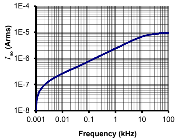
Figure 14: Typical total output rms current noise with R_M = 50 \Omega
