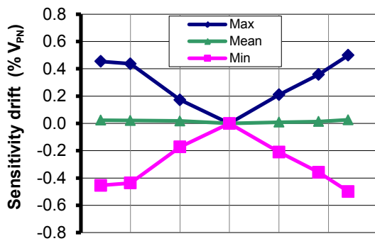
Figure 5: Sensitivity thermal drift
