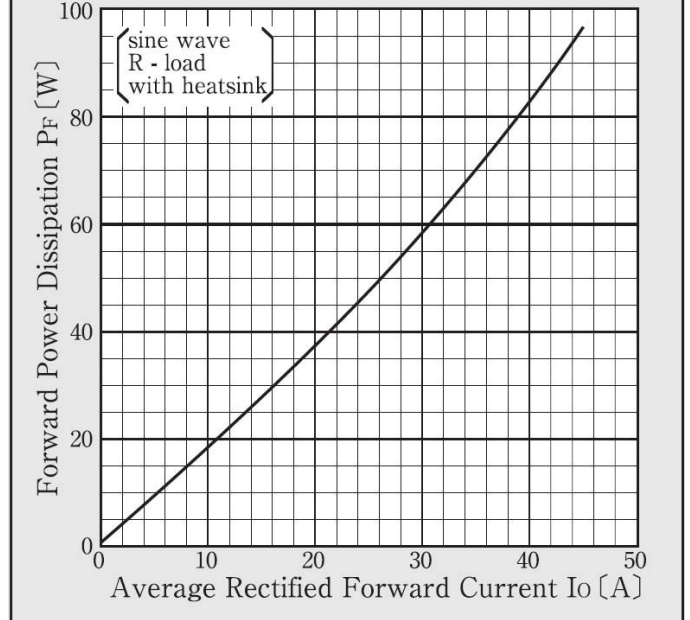
Forward Power Dissipation
