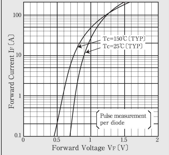
Forward Voltage
