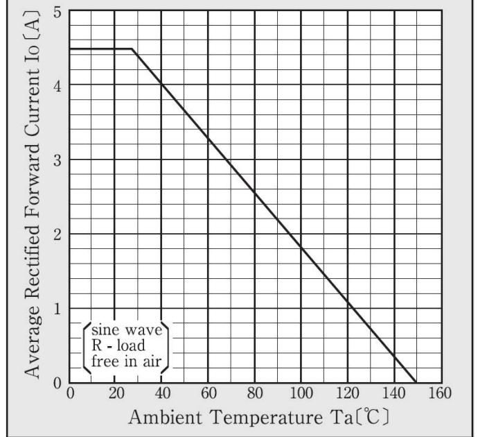
Derating Curve
