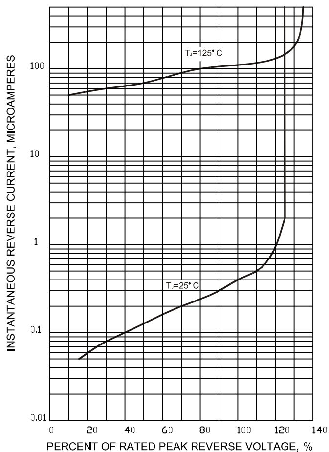
FIG.6-TYPICAL REVERSE CHARACTERISTICS
