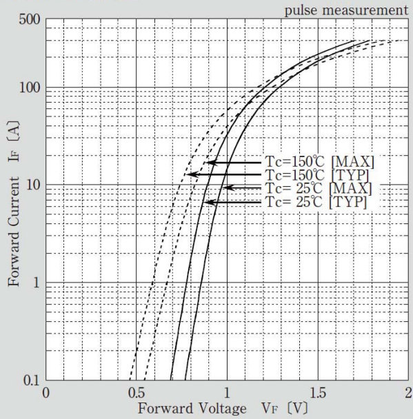
Forward Voltage
