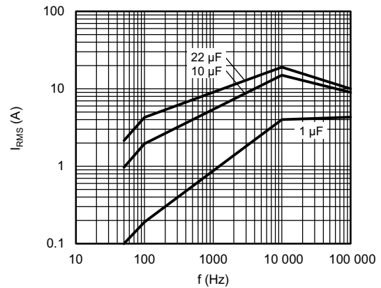
Maximum RMS current as function of frequency T_{amb} \leq 85\text{ }^{\circ}C ; U_n = 310\text{ V}_{AC}
