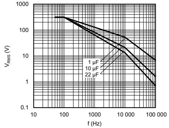
Maximum RMS voltage as function of frequency T_{amb} \leq 85\text{ }^{\circ}C ; U_n = 310\text{ V}_{AC}
