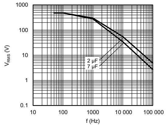
Maximum RMS voltage as function of frequency T_{amb} \leq 85\text{ }^{\circ}C ; U_n = 480\text{ V}_{AC}
