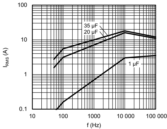
Maximum RMS current as function of frequency T_{amb} \leq 85\text{ }^{\circ}C ; U_n = 250\text{ V}_{AC}
