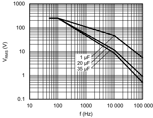
Maximum RMS voltage as function of frequency T_{amb} \leq 85\text{ }^{\circ}C ; U_n = 250\text{ V}_{AC}
