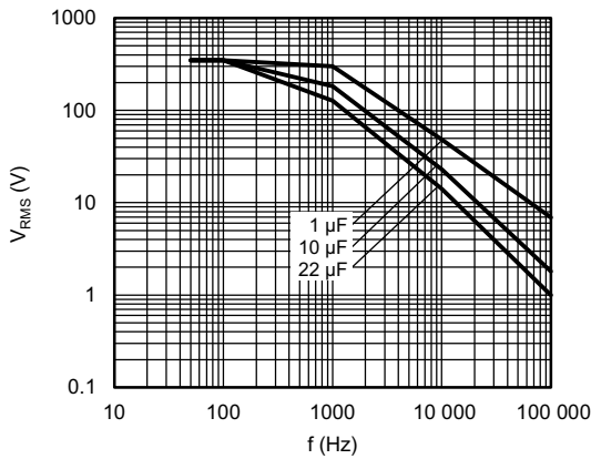
Maximum RMS voltage as function of frequency T_{amb} \leq 85\text{ }^{\circ}C ; U_n = 350\text{ V}_{AC}
