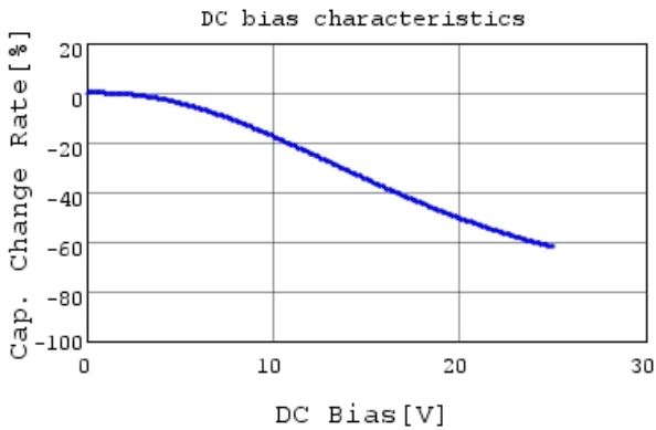
GRT155R71E104KE01 C-DC bias capchange, 25.0c
