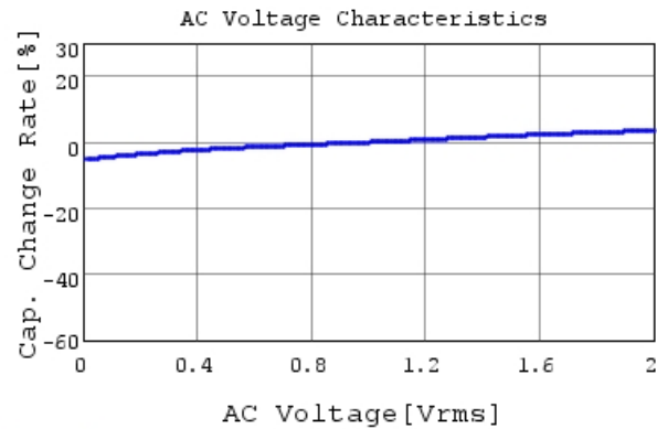
GRT155R71E104KE01 C-AC Voltage capchange, Dc
