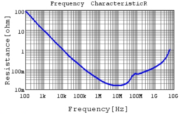
GRT155R71E104KE01 R DCOV,25degC
