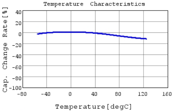
GRT155R71E104KE01 C-Temp. capchange, DC0.0V,
