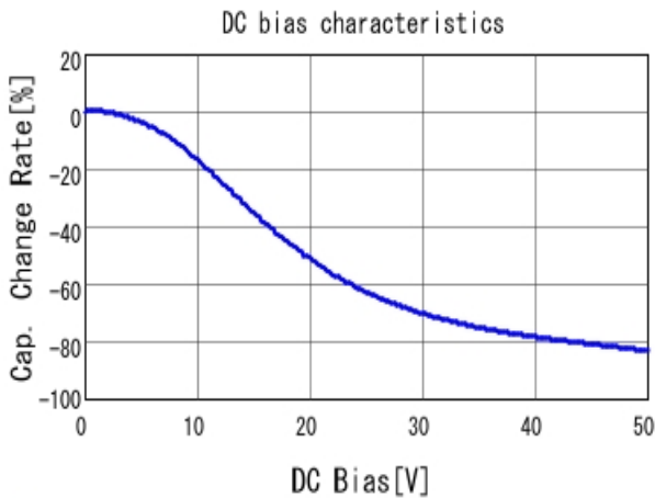
■ GRT155R71H104KE01 C-DC bias capchange, 25.0degC, AC1.
