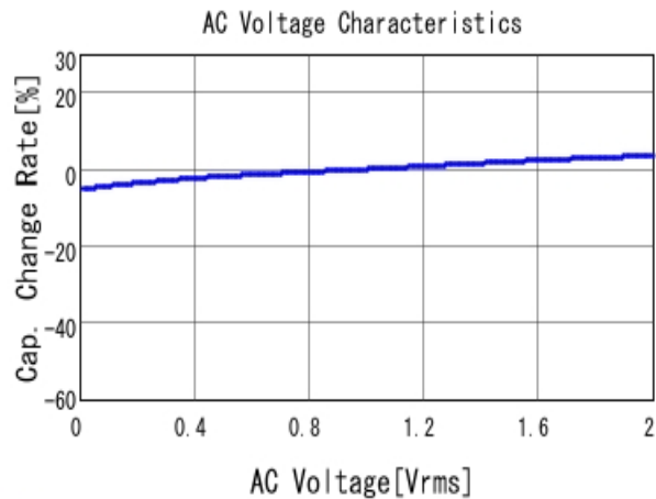
■ GRT155R71H104KE01 C-AC Voltage capchange, DCOV, 25.0d
