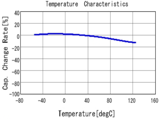
■ GRT155R71H104KE01 C-Temp. capchange, DC0.0V, AC1.0V r m
