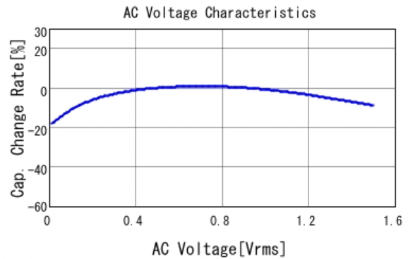
ZRB15XR60J106ME12 C-AC Voltage capchange, DC0V, 25.0d
