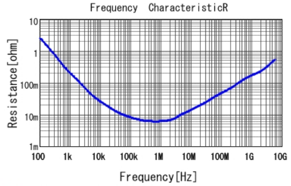
ZRB15XR60J106ME12 R DC0V, 25degC
