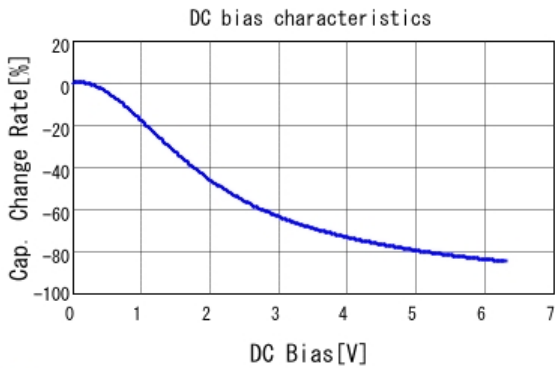
ZRB15XR60J106ME12 C-DC bias capchange, 25.0degC, AC0.
