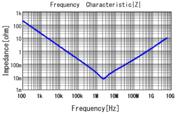
ZRB15XR60J106ME12 |Z| DC0V, 25degC
