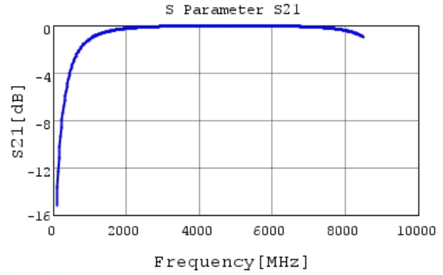
GJM1555C1H2R8WB01 S21 DCOV, 25degC
