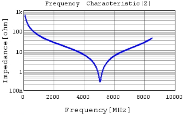
GJM1555C1H2R8WB01 |Z| DC0V, 25degC
