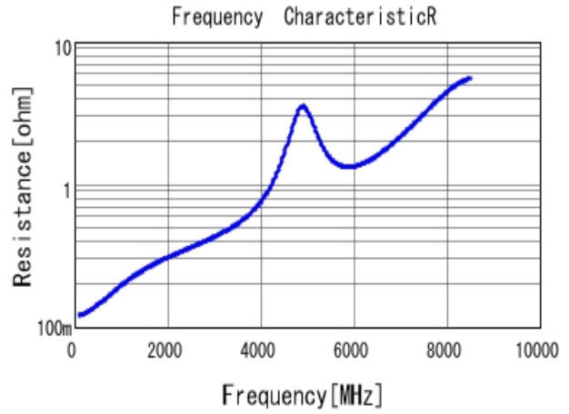
■ GRM1555C1H120GA01 R DCOV, 25degC
