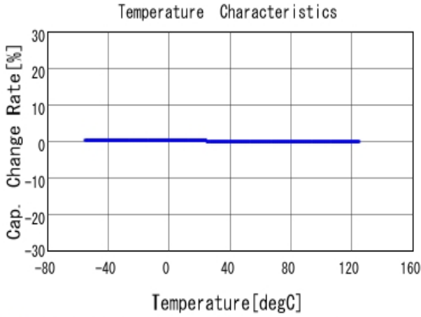
■ GRM1555C1H120GA01 C-Temp. capchange, DCOV, AC1Vrms
