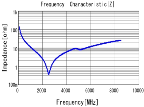
■ GRM1555C1H120GA01 |Z| DCOV, 25degC
