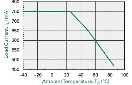
Maximum Load Current vs. Temperature ( I_F = 2 \text{ mA} )
