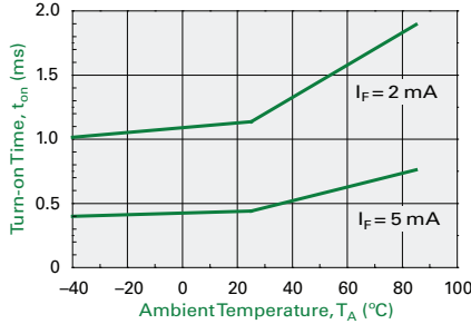
Typical Turn-on Time vs. Temperature (I L = 100 mA)
