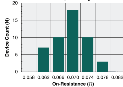
Typical On-Resistance Distribution (N=50, I_F=5\text{mA} , I_L=1\text{A} )
