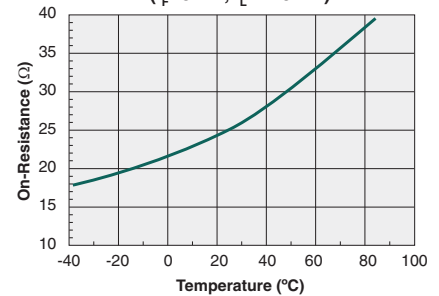
Typical On-Resistance vs. Temperature ( I_F=5\text{mA} , I_L=120\text{mA} )
