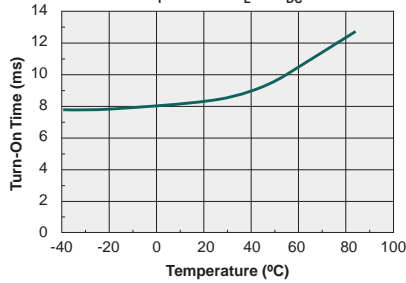
Typical Turn-On Time vs. Temperature ( I_F=10\text{mA} , I_L=1\text{A}_{DC} )
