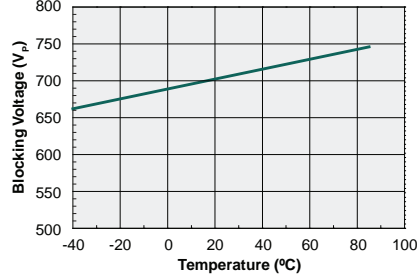
Typical Blocking Voltage vs. Temperature
