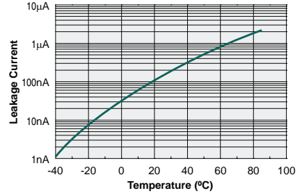
Typical Leakage vs. Temperature Measured Across Pins 1&2 ( V_L=600\text{V} )
