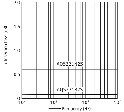
15.Insertion loss vs. frequency characteristics (50Ω impedance)
