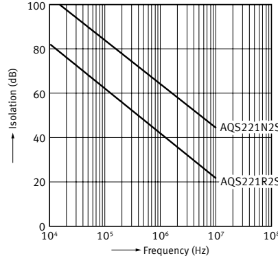
14.Isolation vs. frequency characteristics (50Ω impedance)
