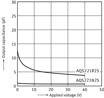
13.Output capacitance vs. applied voltage characteristics
