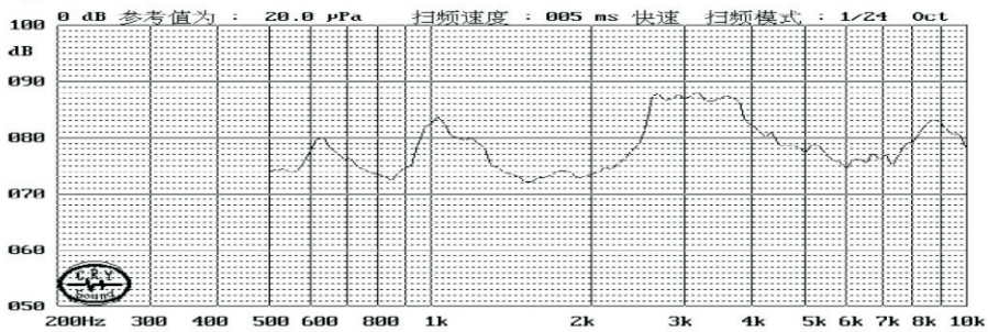
TYPICAL FREQUENCY RESPONSE CURVE 频率曲线
