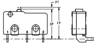
Operate Point References for PCB Terminals
