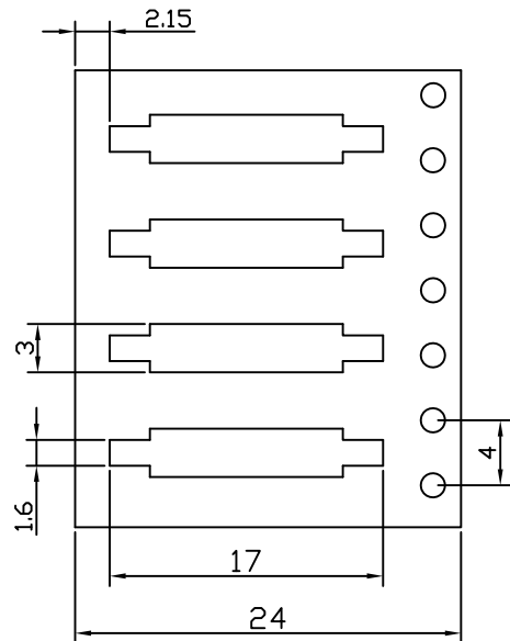
卷盘包装尺寸 Dimensions for tape and reel
