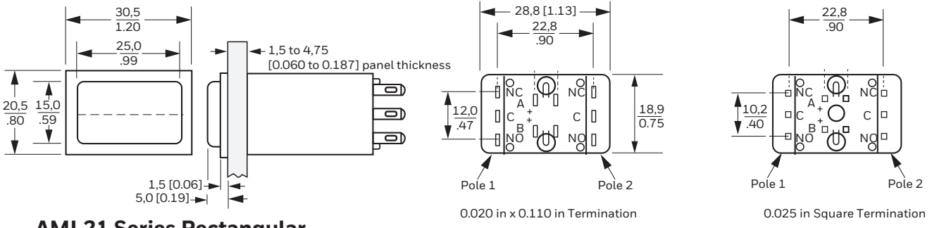
AML21 Series Rectangular
