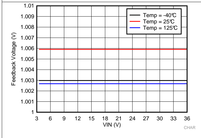
Figure 3. Feedback Voltage
