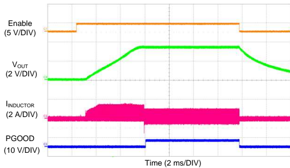
Figure 75. LM73606-Q1 Overcurrent Behavior
