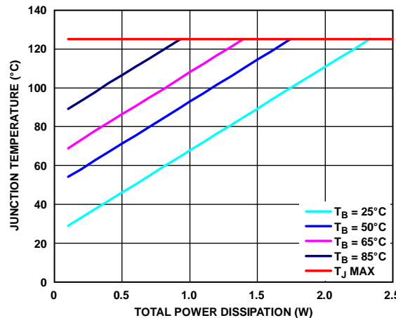
Figure 63. TSOT Junction Temperature Rise, Different Board Temperatures
