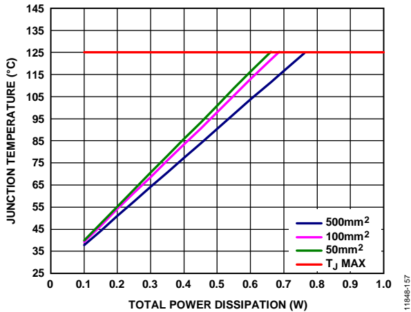
Figure 58. TSOT, T_A = 25^\circ\text{C}
