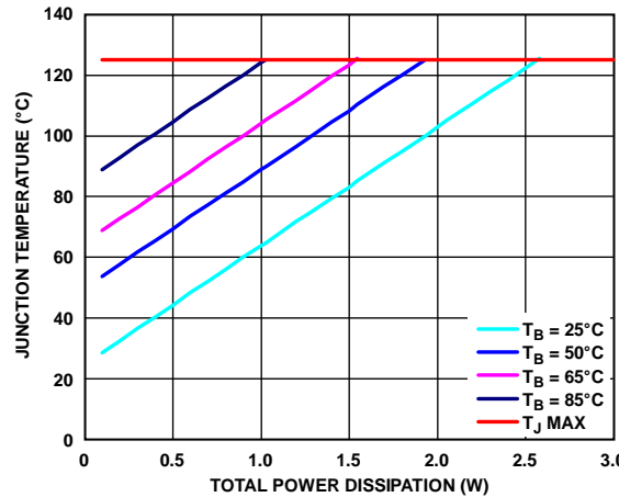
Figure 62. SOIC Junction Temperature Rise, Different Board Temperatures
