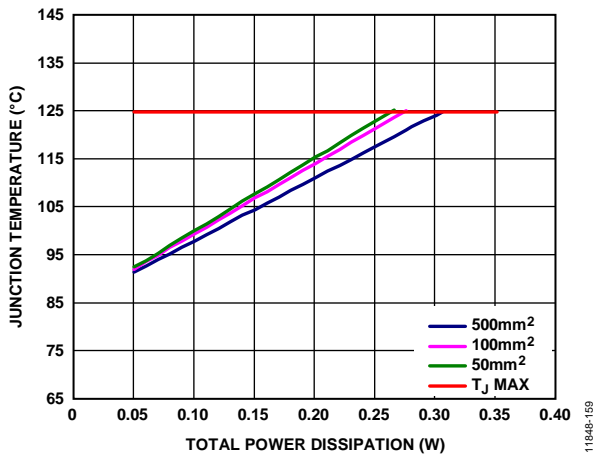
Figure 60. TSOT, T_A = 85^\circ\text{C}
