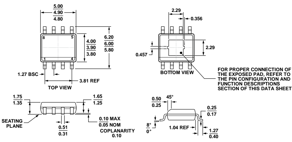
COMPLIANT TO JEDEC STANDARDS MS-012-AA Figure 68. 8-Lead Standard Small Outline Package, with Exposed Pad [SOIC_N_EP] Narrow Body (RD-8-1) Dimensions shown in millimeters
