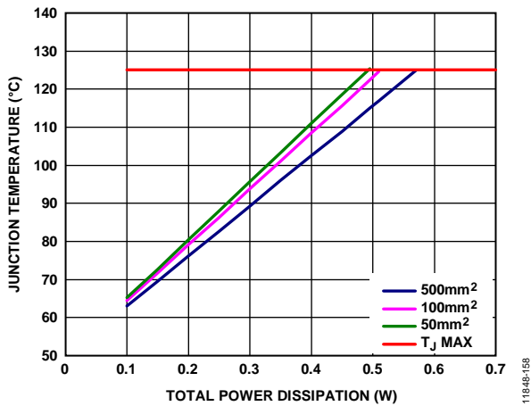
Figure 59. TSOT, T_A = 50^\circ\text{C}
