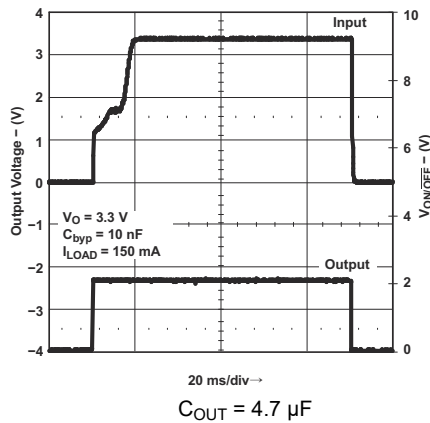
Figure 8-23. Turn-On Time
