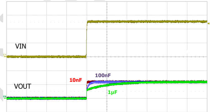
VIN : 1.0V/div, VOUT : 1.0V/div, Time : 10ms/div Start Up @ I out =10mA
