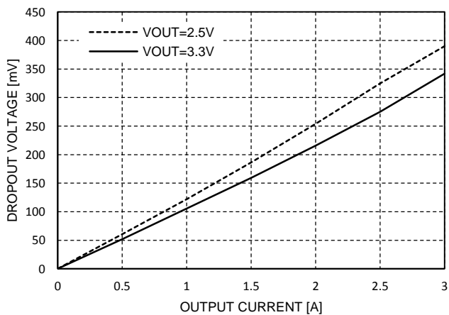
Dropout Voltage
