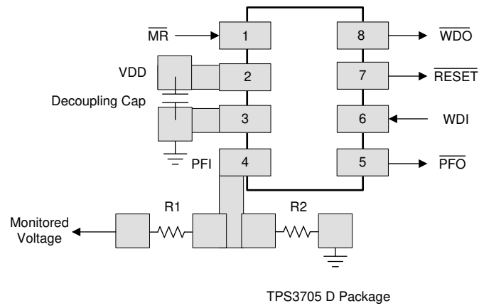
Figure 11-1. TPS3705 Layout
